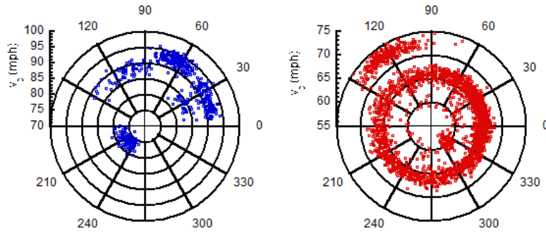
Figure 3. Polar scatter plot of movement direction in the x-z plane versus release speed for normal pitcher Jon Lester (left) and knuckleball pitcher Tim Wakefield (right). The knuckleballs are in the ring centered at 66 mph. Whereas the normal pitches are clustered in angle and speed, the direction of the knuckleball movement appears to be completely random.
