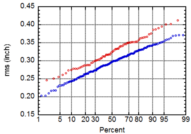
Figure 1 Distribution of rms values for normal (blue) and knuckleball (red) pitches. The nearly parallel linear contours of these samples indicate that they each have a Gaussian distribution with the same standard deviation but with the mean value slightly larger for knuckleballs.
