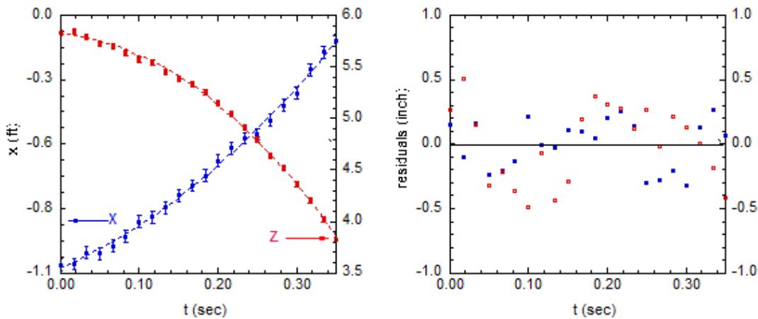
Figure 2. Trajectory of a knuckleball pitch (left) along with the fit. The error flags are 0.025 ft. The right plot shows the difference between the actual and fitted values. The rms deviation of the fit from the data is 0.39 inch, demonstrating the smoothness of the trajectory.
