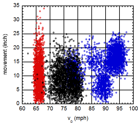
Figure 4 Scatter plot of total movement versus release speed for Wakefield (red), Dickey (black), and Lester (blue). This plot shows that the knuckleball movement is as random in magnitude as it is in direction.
